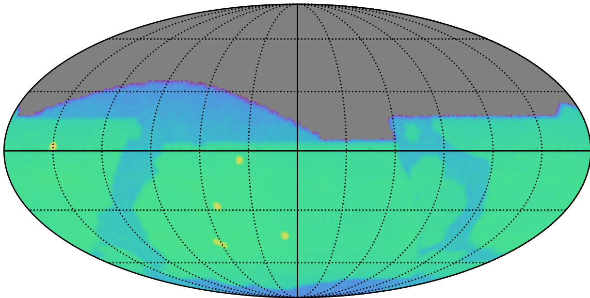
too_10_1v3.4_10yrs z: CoaddM5
