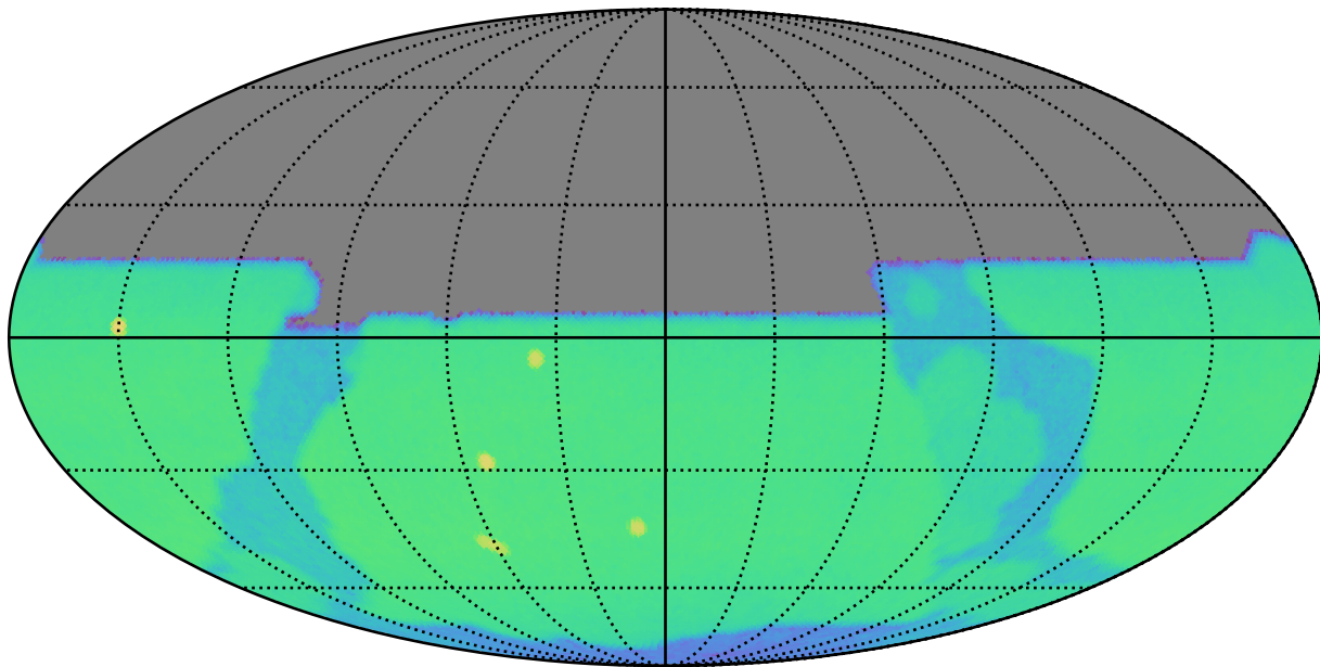
too_10_1v3.4_10yrs y: CoaddM5
