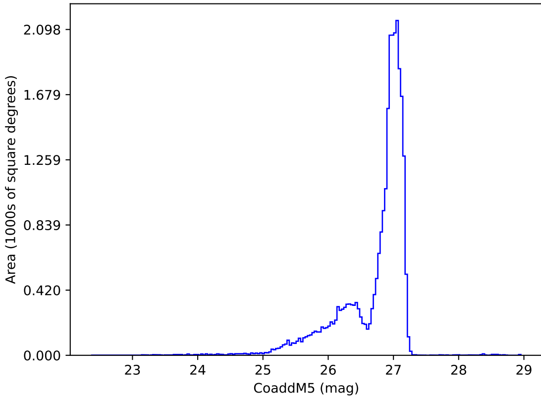
too_10_1v3.4_10yrs r: CoaddM5
