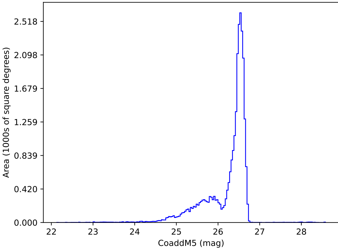
too_10_1v3.4_10yrs i: CoaddM5
