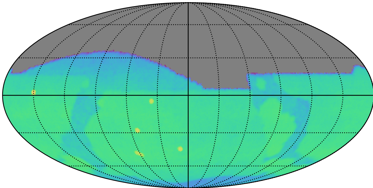
too_10_1v3.4_10yrs g: CoaddM5
