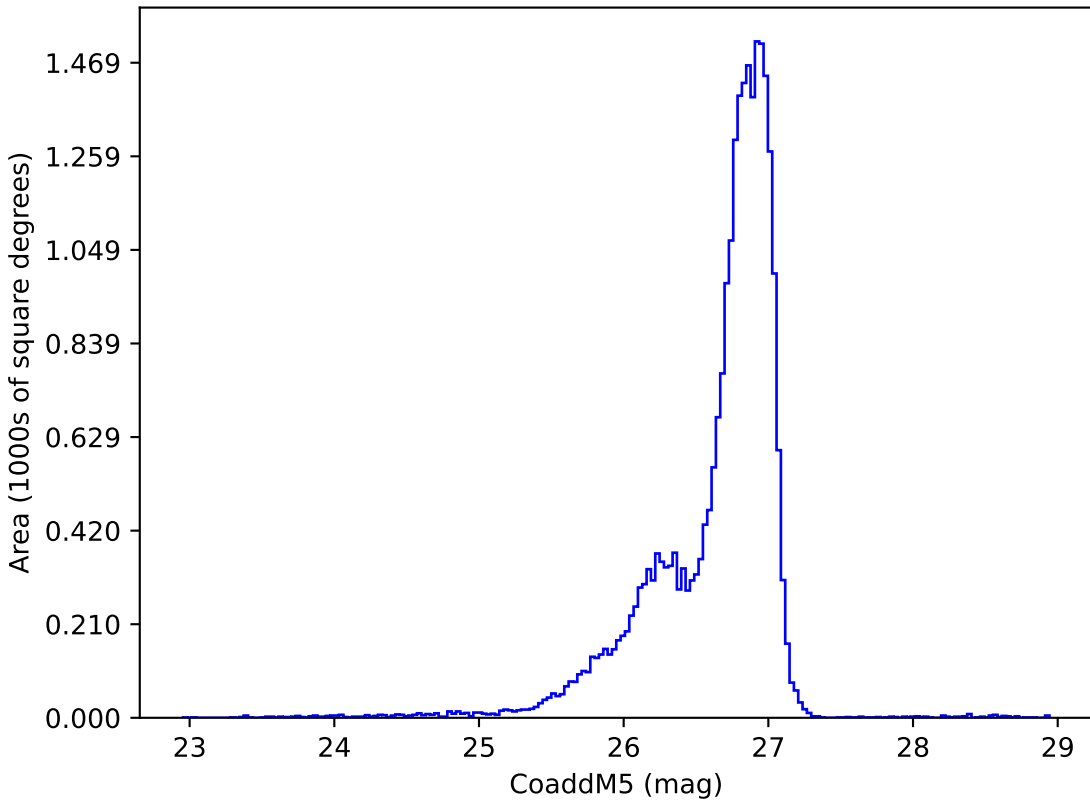
too_10_1v3.4_10yrs g: CoaddM5
