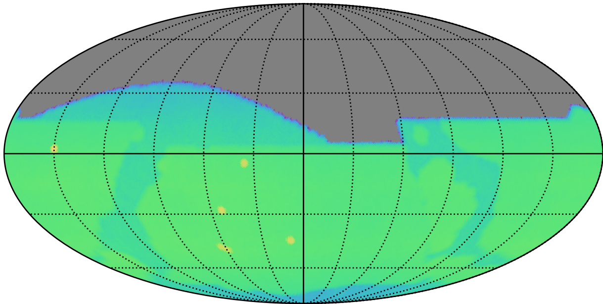
too_10_1v3.4_10yrs : CoaddM5
