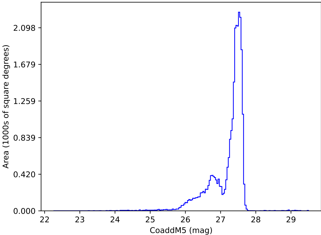
too_10_1v3.4_10yrs : CoaddM5
