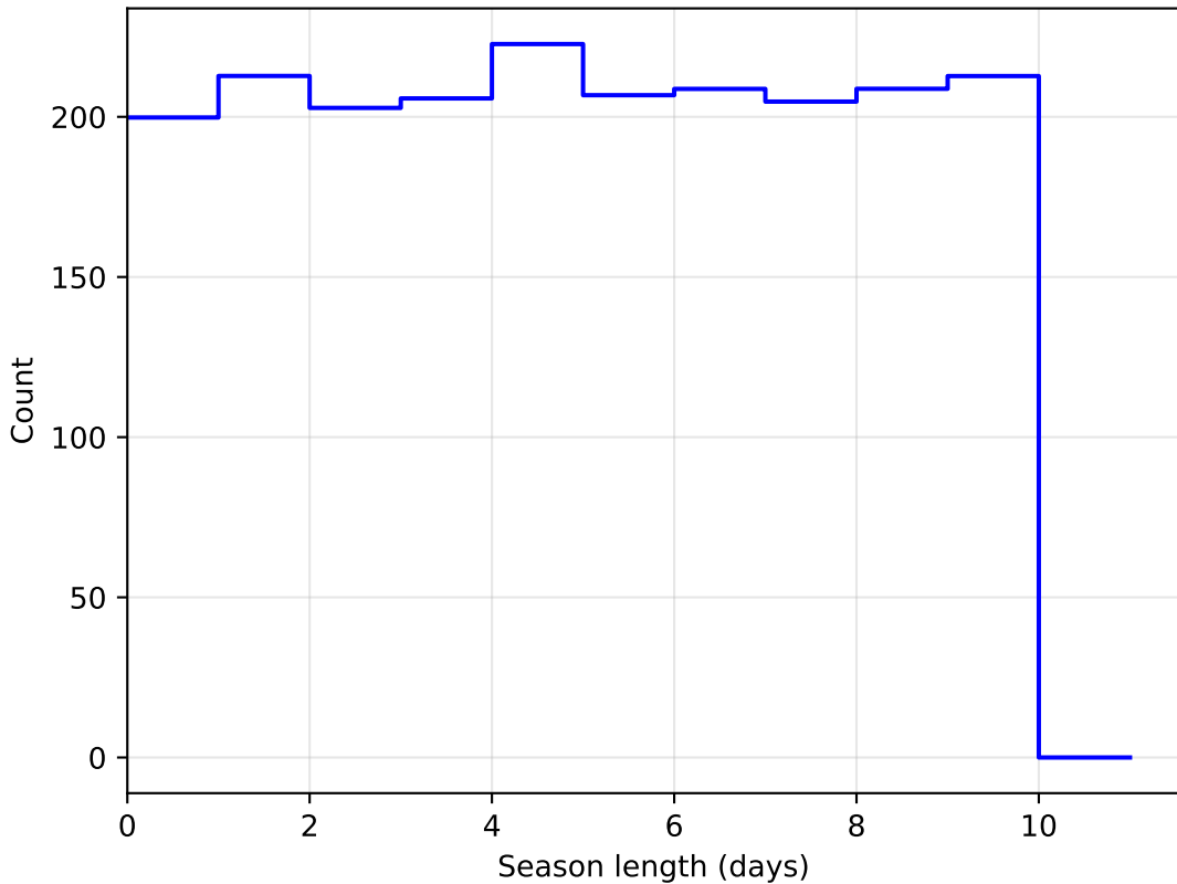
too_10_1v3.4_10yrs DD:XMM_LSS all bands: SeasonLength
