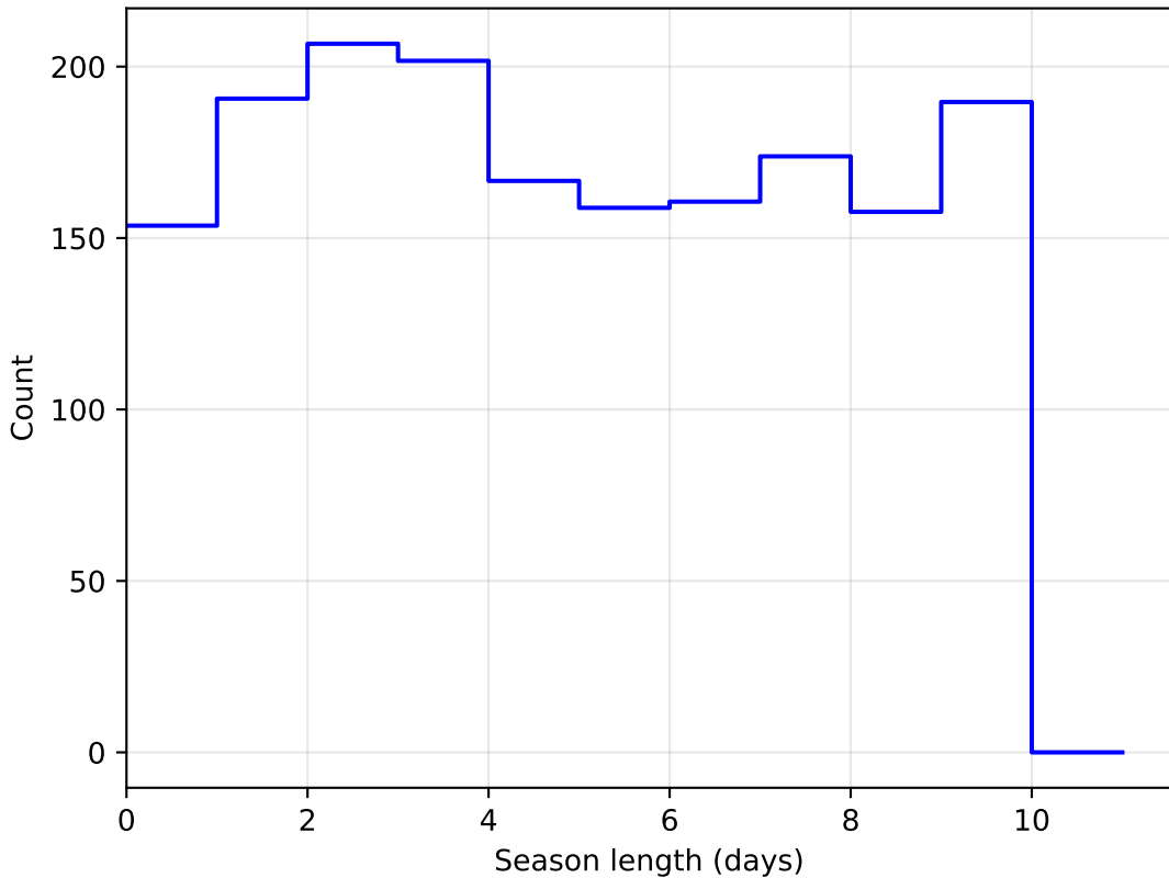
too_10_1v3.4_10yrs DD:WFD all bands: SeasonLength
