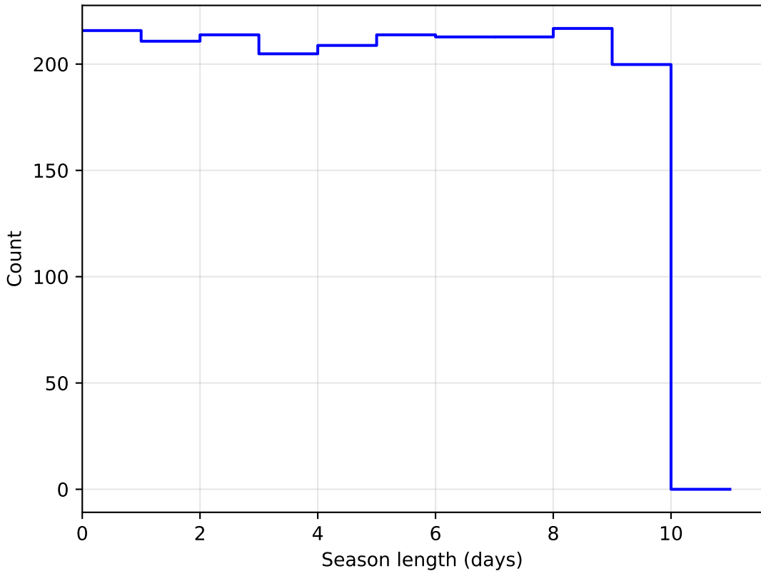
too_10_1v3.4_10yrs DD:ECDFS all bands: SeasonLength
