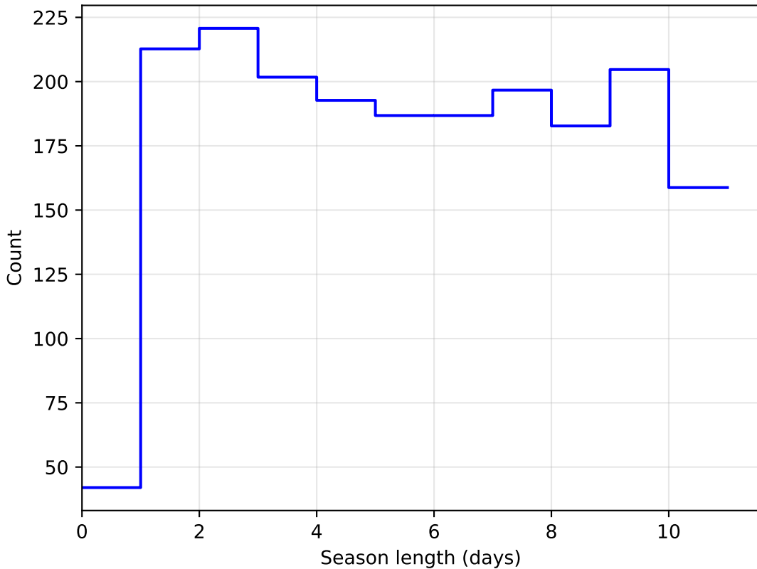
too_10_1v3.4_10yrs DD: COSMOS all bands: SeasonLength
