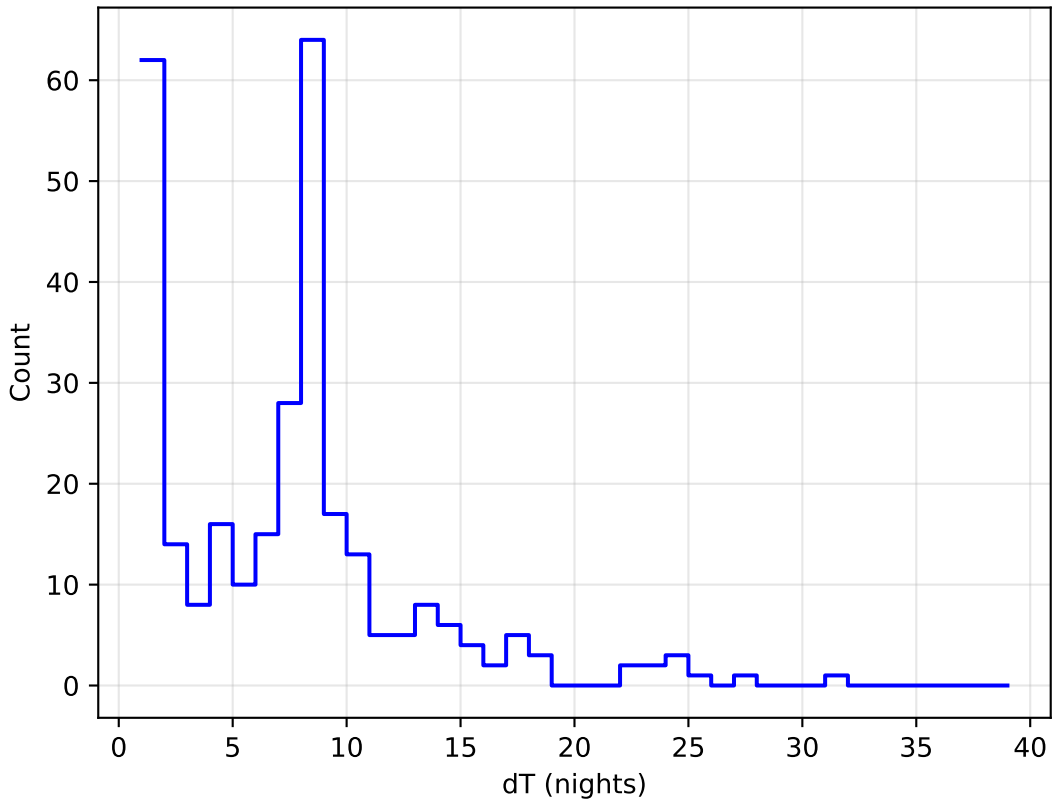
too_10_1v3.4_10yrs all bands: DD:XMM_LSS Delta Nights Histogram
