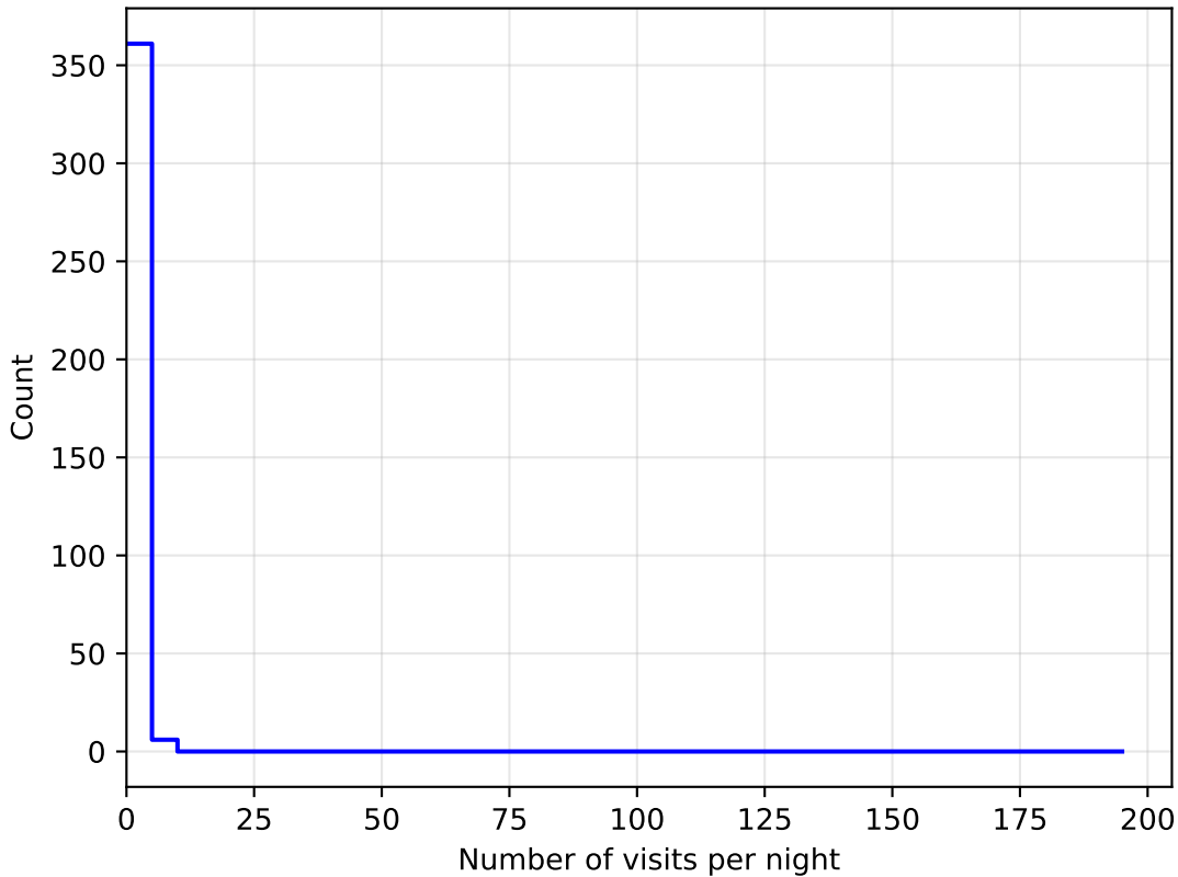
too_10_1v3.4_10yrs all bands: DD:WFD NVisitsPerNight
