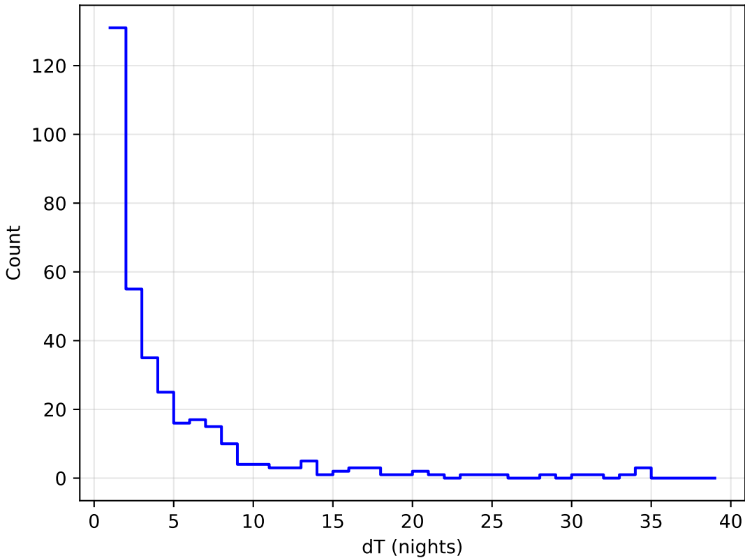
too_10_1v3.4_10yrs all bands: DD:WFD Delta Nights Histogram
