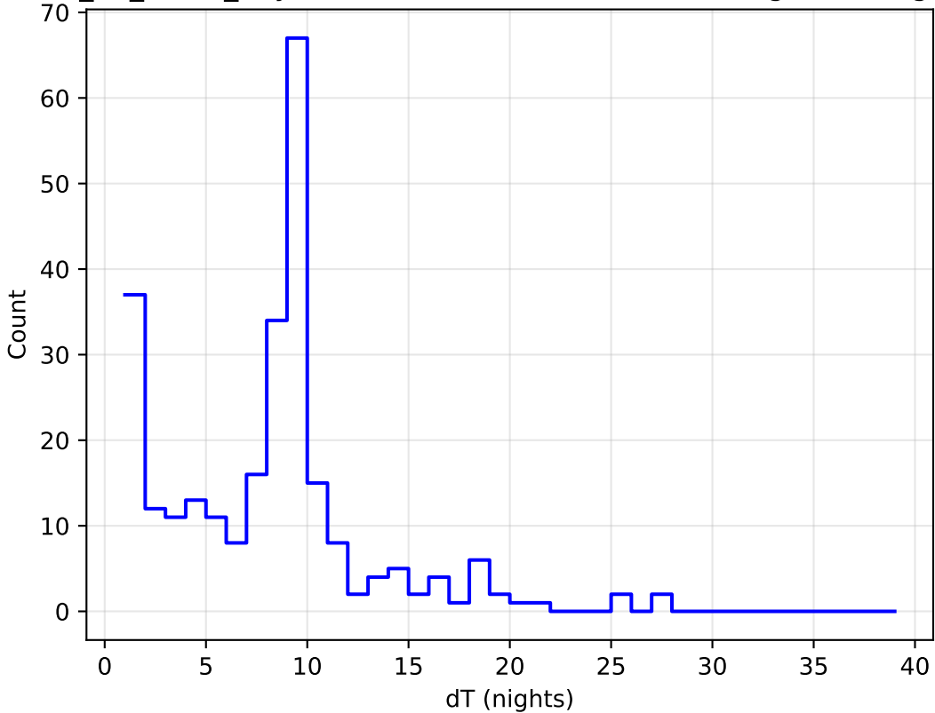
too_10_1v3.4_10yrs all bands: DD:ELAISS1 Delta Nights Histogram
