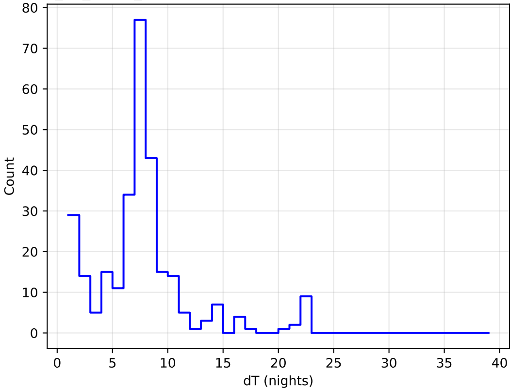
too_10_1v3.4_10yrs all bands: DD:EDFS Delta Nights Histogram
