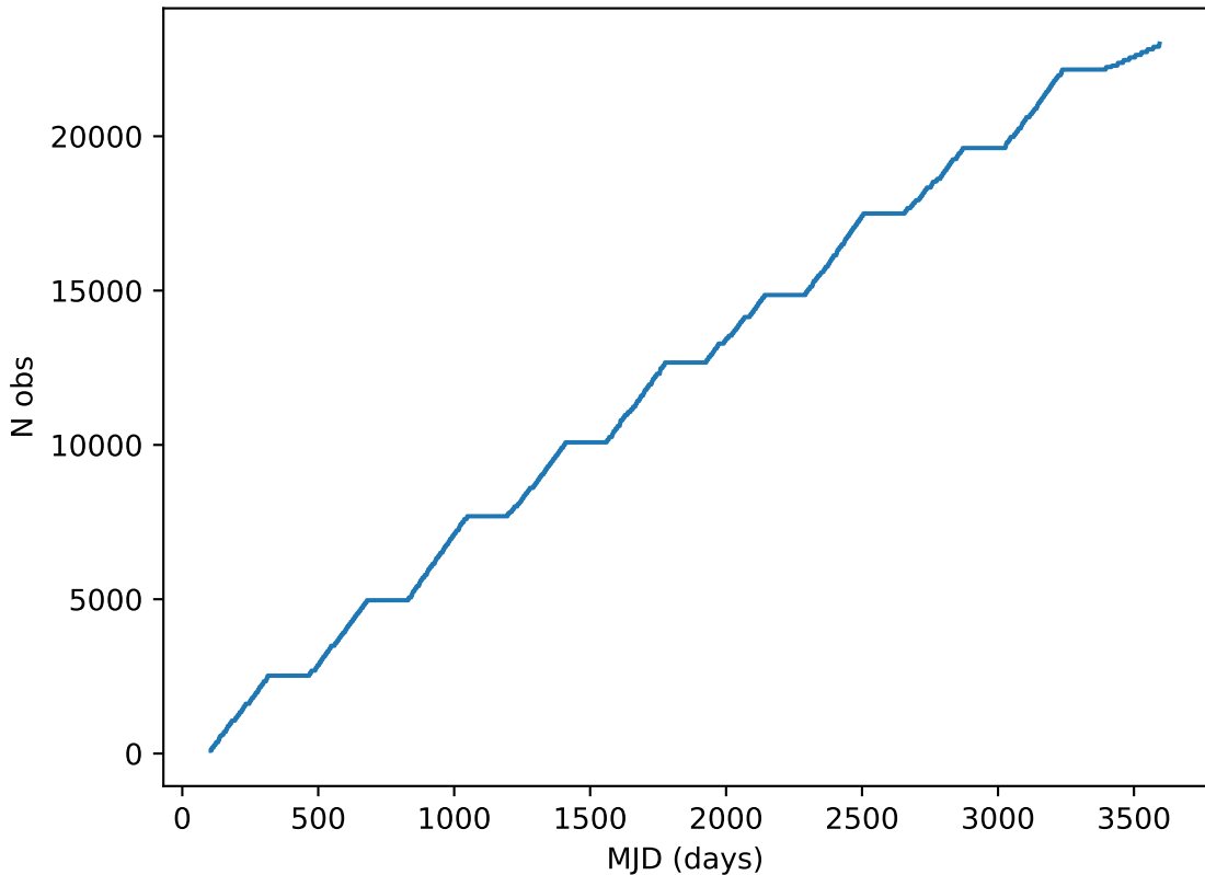
too_10_1v3.4_10yrs all bands: DD:EDFS Cumulative NVisits
