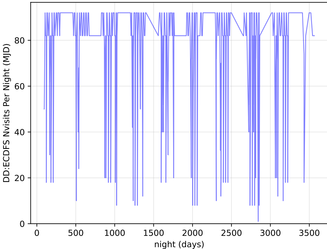
too_10_1v3.4_10yrs all bands: DD:ECDFS Nvisits Per Night
