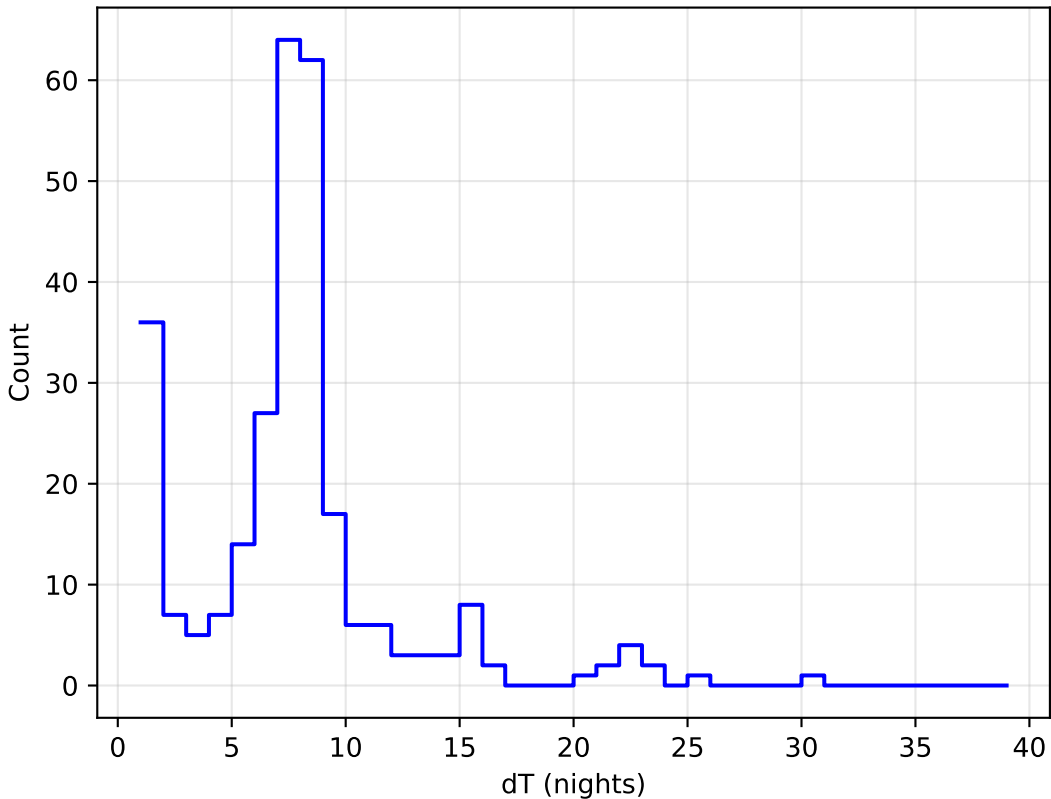
too_10_1v3.4_10yrs all bands: DD:ECDFS Delta Nights Histogram
