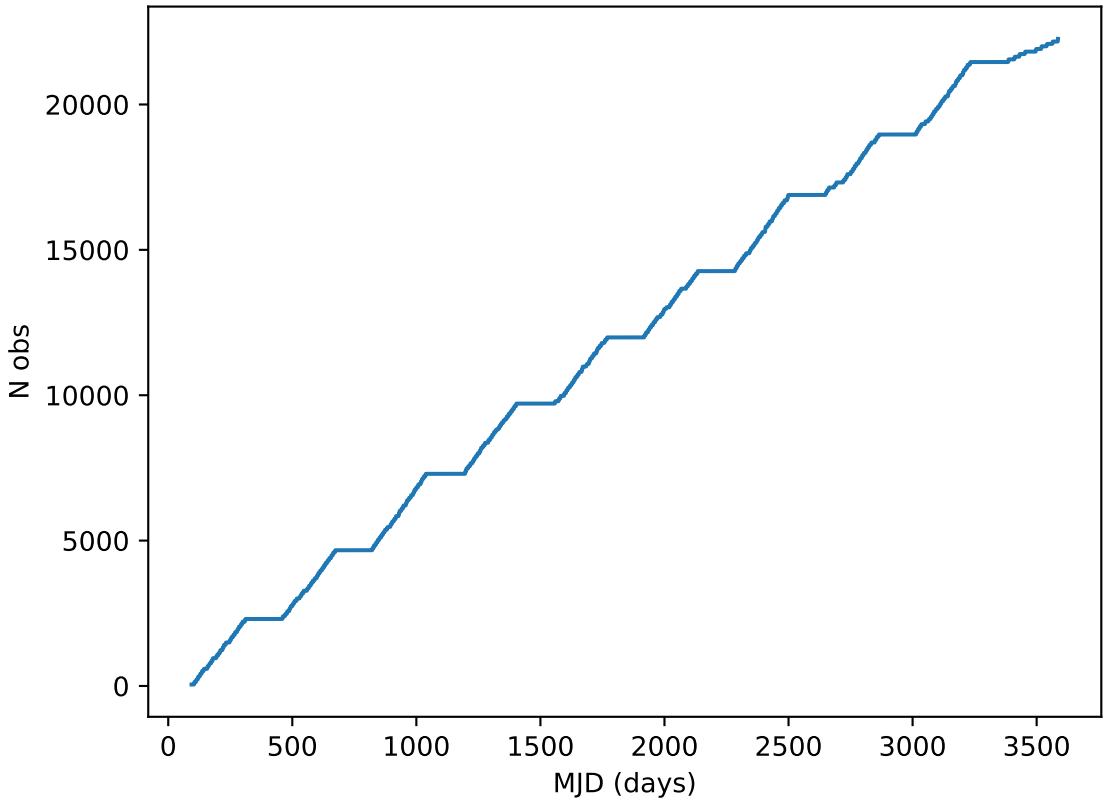
too_10_1v3.4_10yrs all bands: DD:ECDFS Cumulative NVisits
