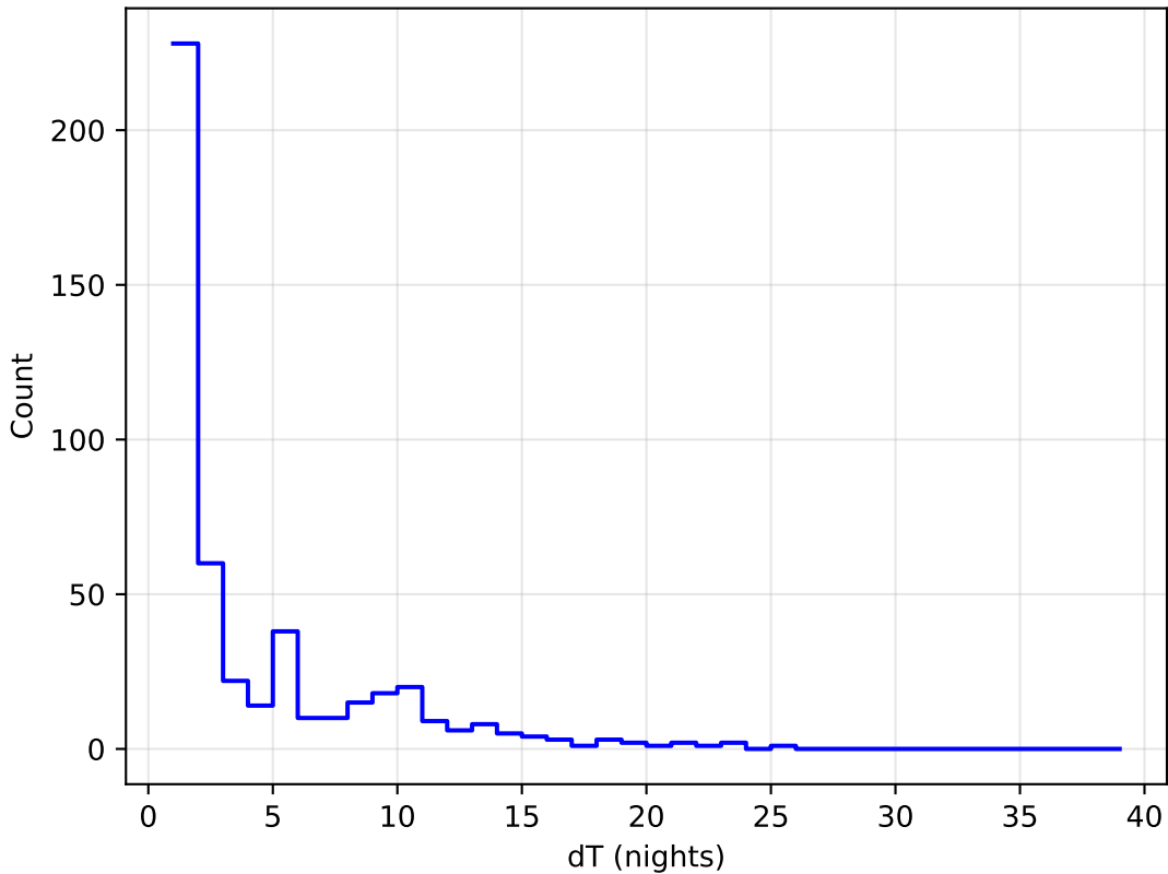
too_10_1v3.4_10yrs all bands: DD: COSMOS Delta Nights Histogram
