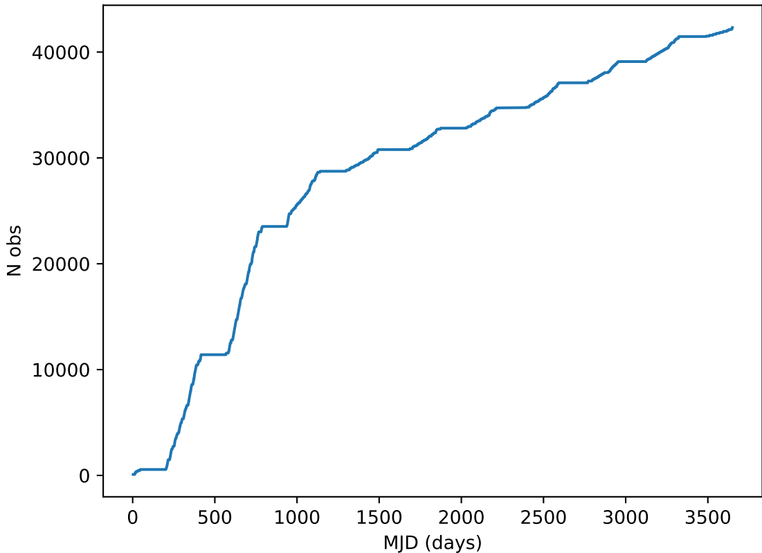
too_10_1v3.4_10yrs all bands: DD:COSMOS Cumulative NVisits
