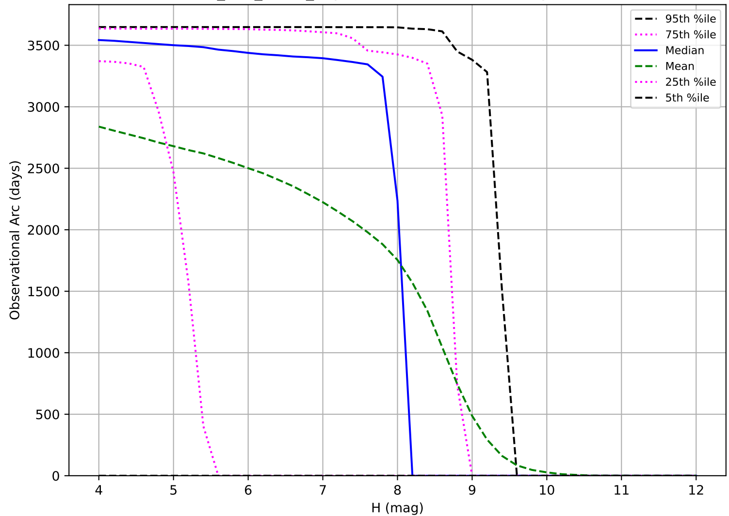
too_100_4v3.4_10yrs: Observational Arc Length TNO
