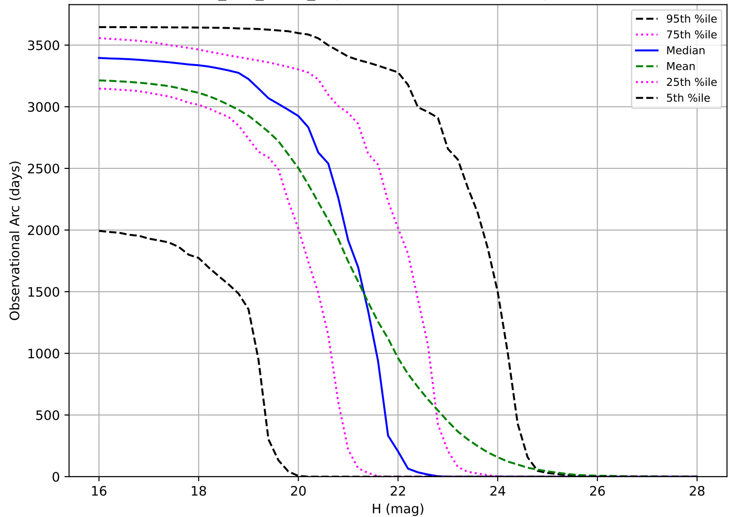
too_100_4v3.4_10yrs: Observational Arc Length PHA
