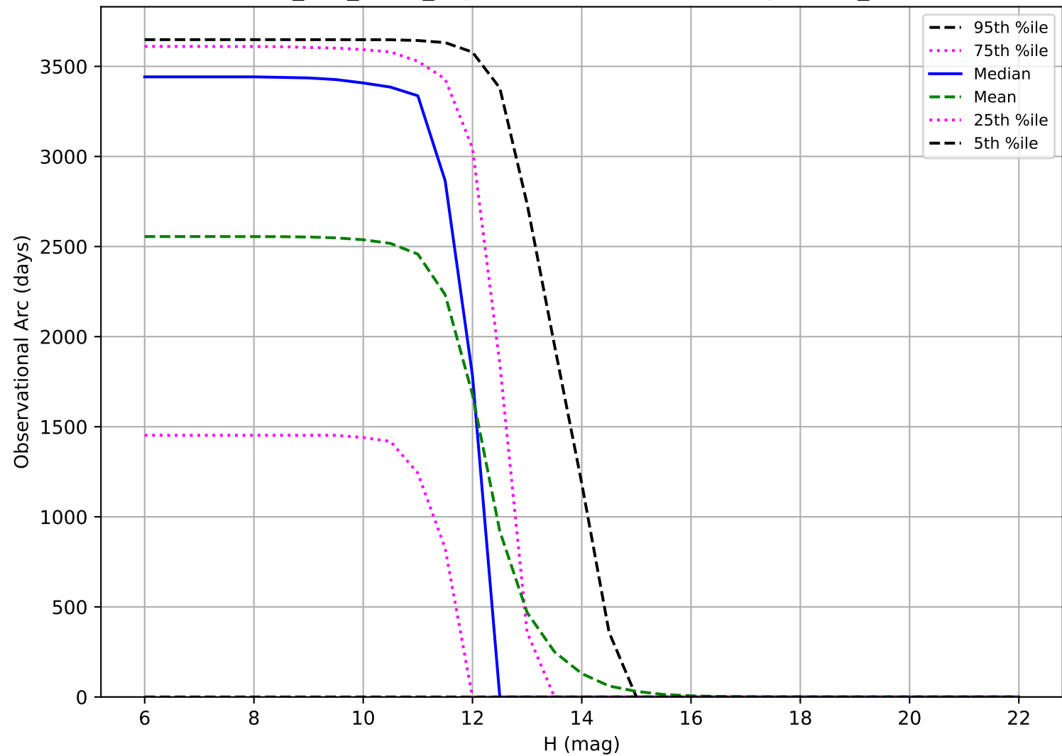
too_100_4v3.4_10yrs: Observational Arc Length OCC_r20
