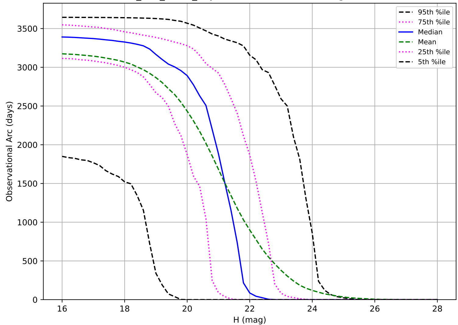
too_100_4v3.4_10yrs: Observational Arc Length NEO
