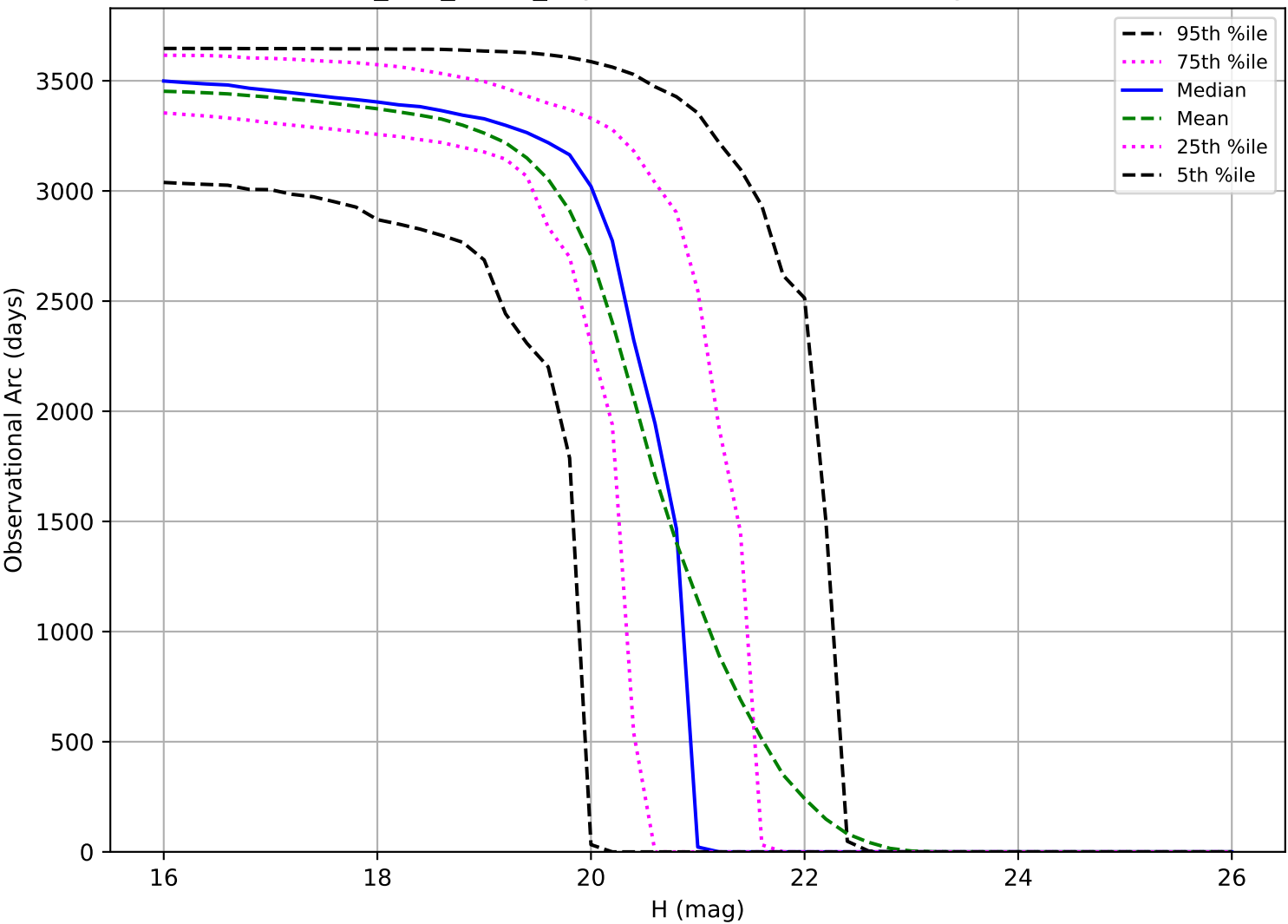
too_100_4v3.4_10yrs: Observational Arc Length MBA
