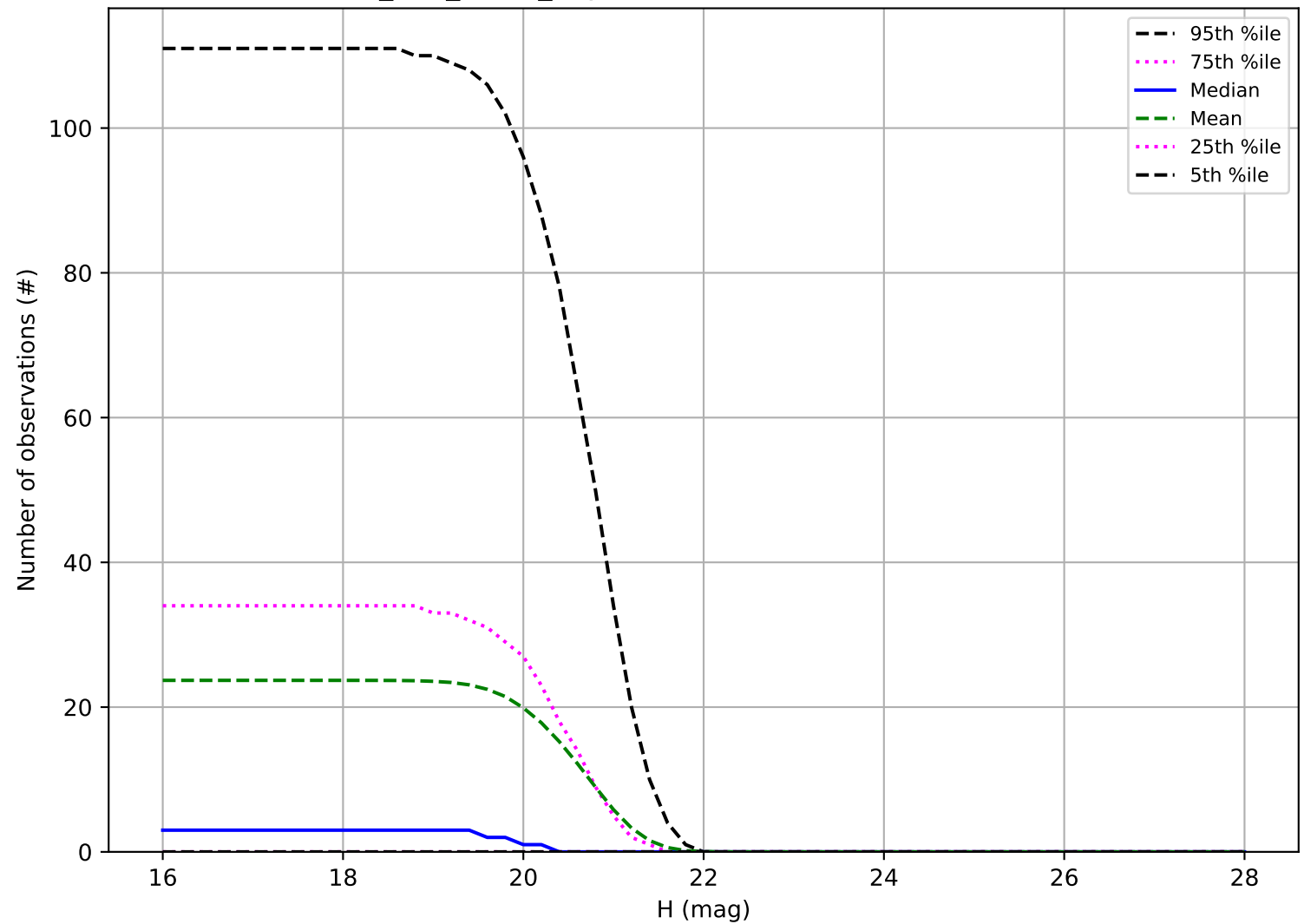
too_100_4v3.4_10yrs: Number of observations Vatira
