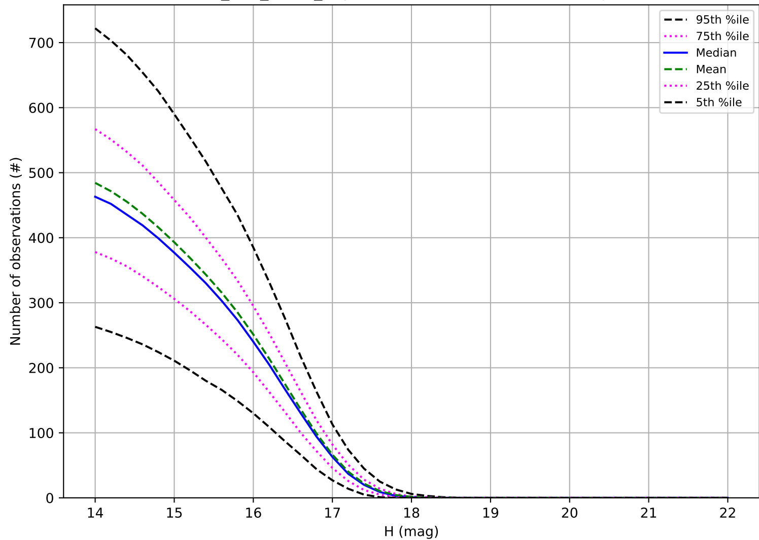
too_100_4v3.4_10yrs: Number of observations Trojan
