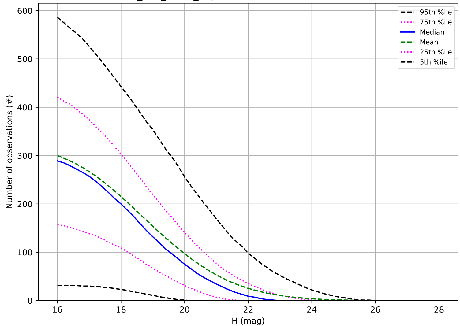
too_100_4v3.4_10yrs: Number of observations NEO
