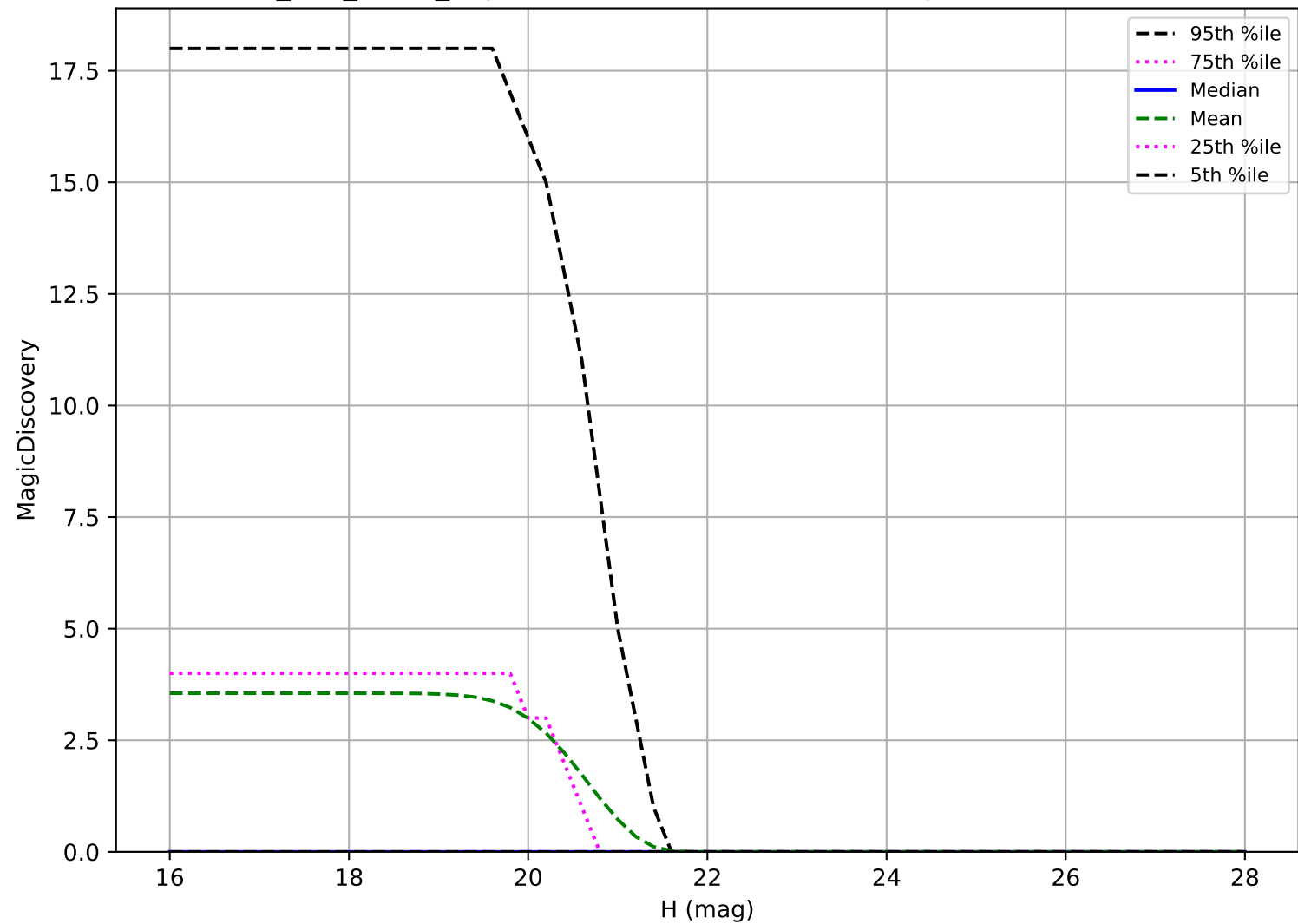
too_100_4v3.4_10yrs: Vatira 6 detections in 60 nights detection loss
