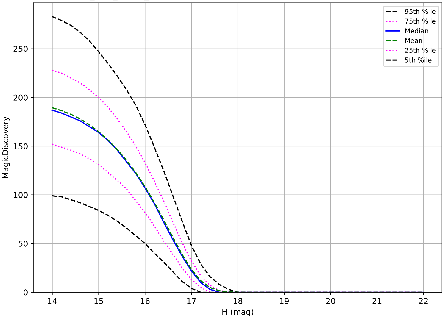
too_100_4v3.4_10yrs: Trojan 6 detections in 60 nights detection loss
