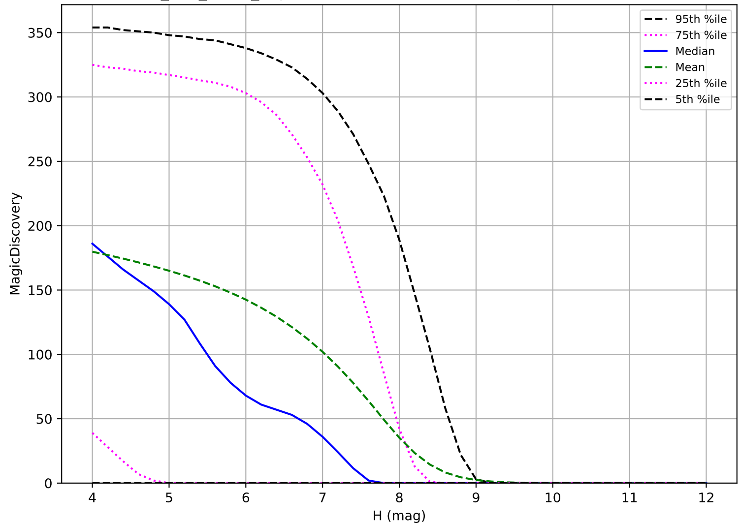
too_100_4v3.4_10yrs: TNO 6 detections in 60 nights detection loss
