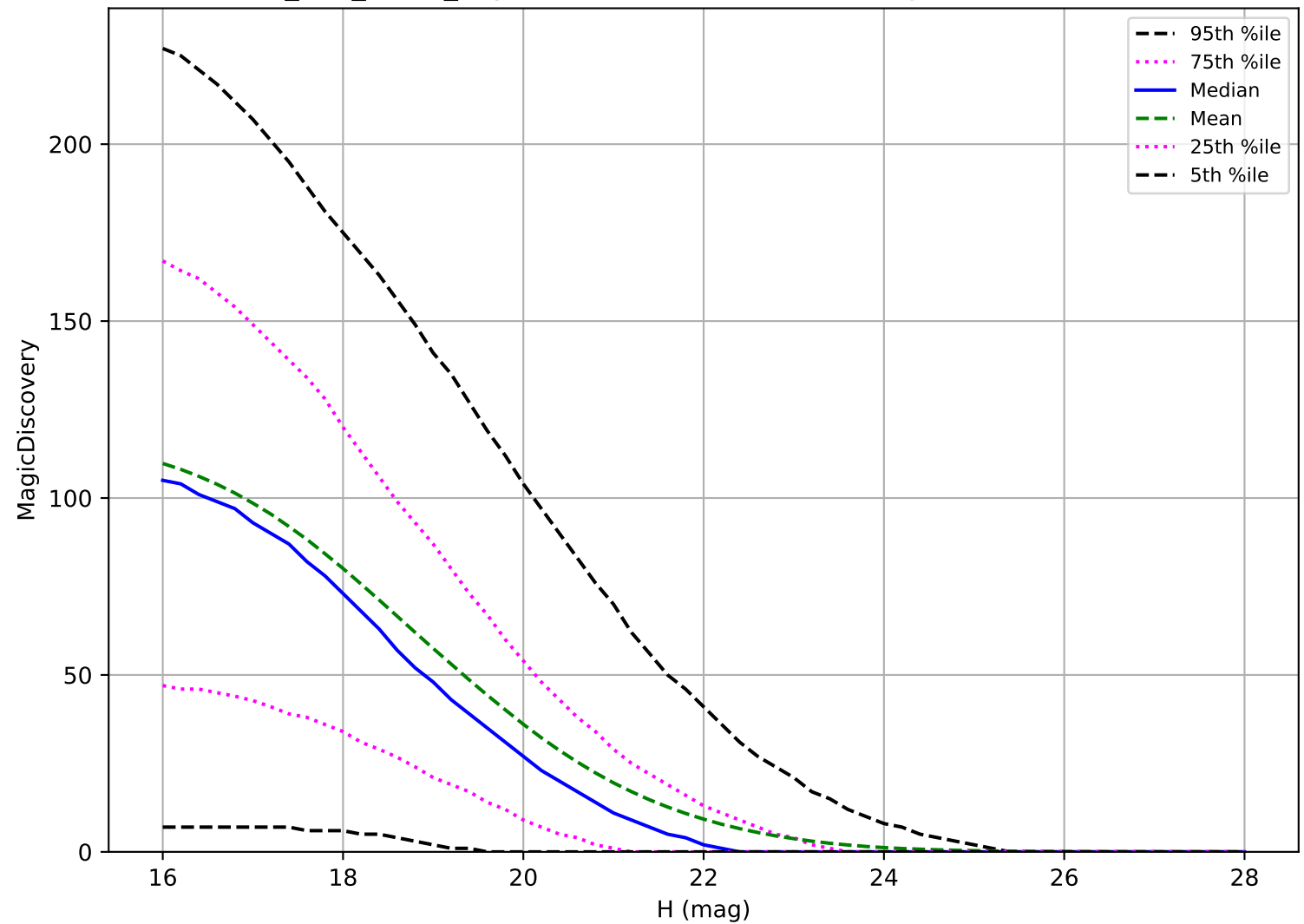
too_100_4v3.4_10yrs: PHA 6 detections in 60 nights detection loss
