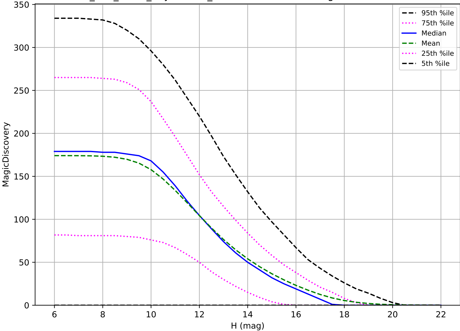
too_100_4v3.4_10yrs: OCC_r5 6 detections in 60 nights detection loss
