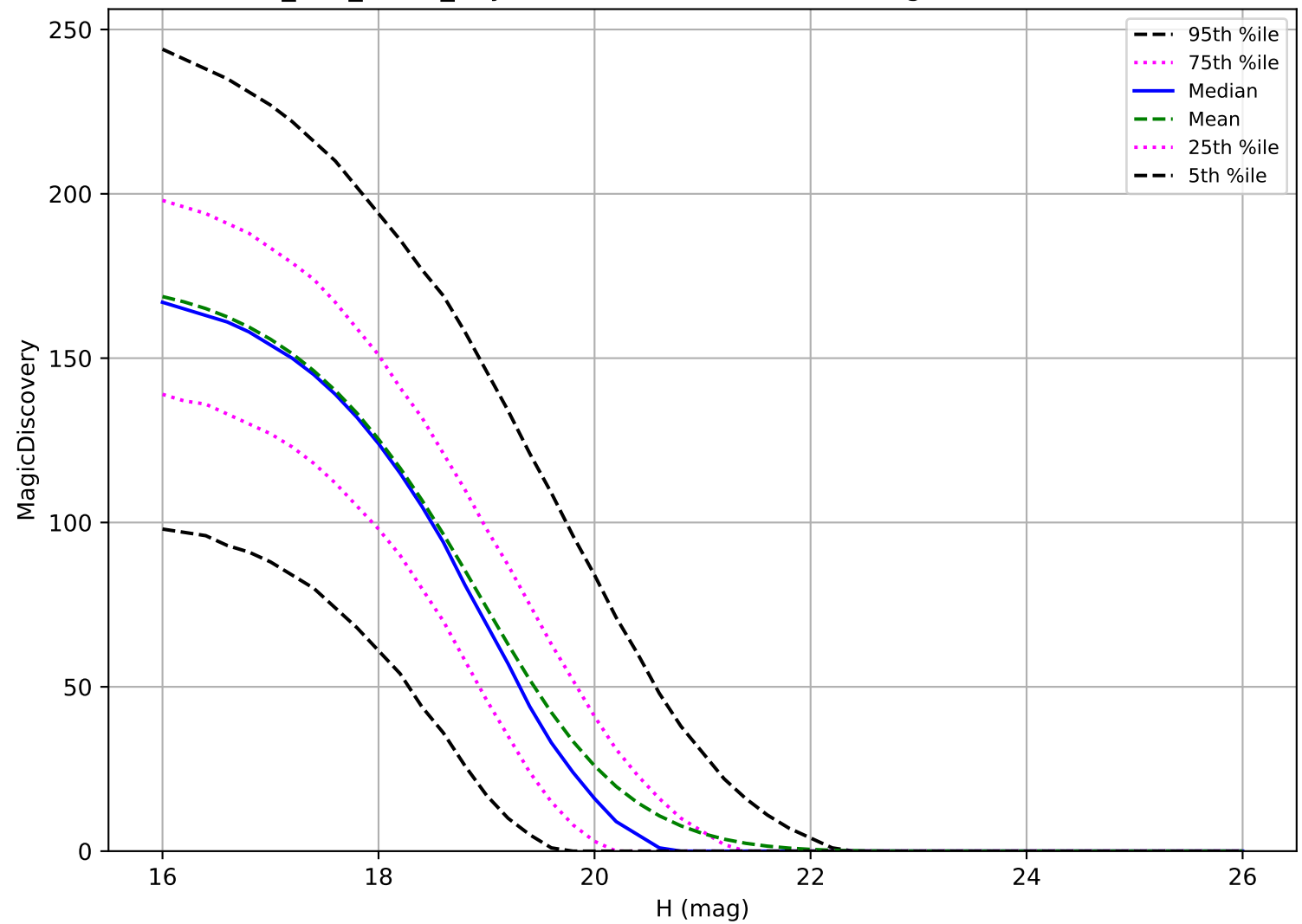
too_100_4v3.4_10yrs: MBA 6 detections in 60 nights detection loss
