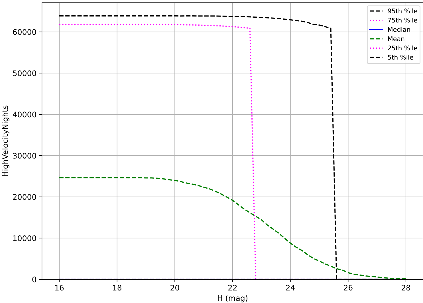
too_100_4v3.4_10yrs: PHA High velocity pair detection loss
