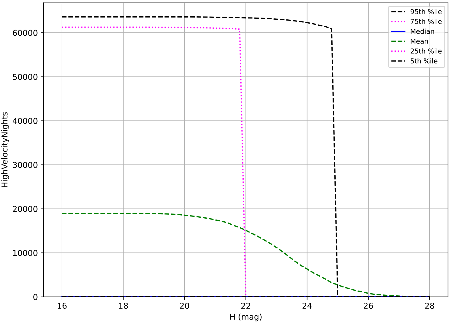
too_100_4v3.4_10yrs: NEO High velocity pair detection loss
