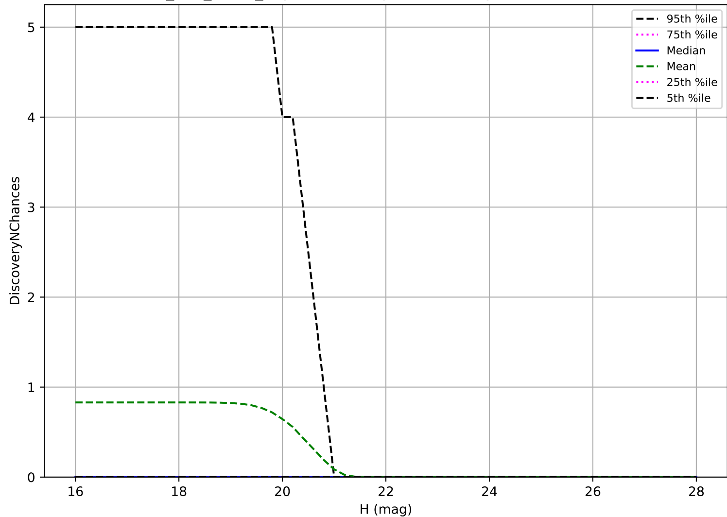
too_100_4v3.4_10yrs: Vatira 3 pairs in 15 nights detection loss
