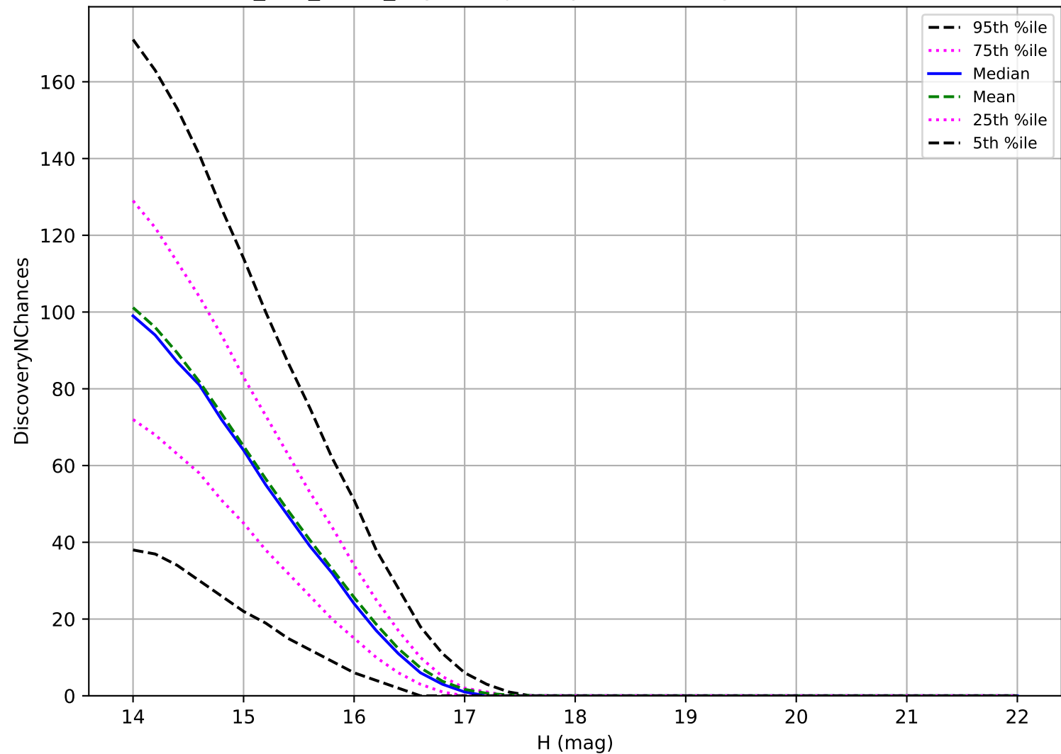
too_100_4v3.4_10yrs: Trojan 3 pairs in 15 nights detection loss
