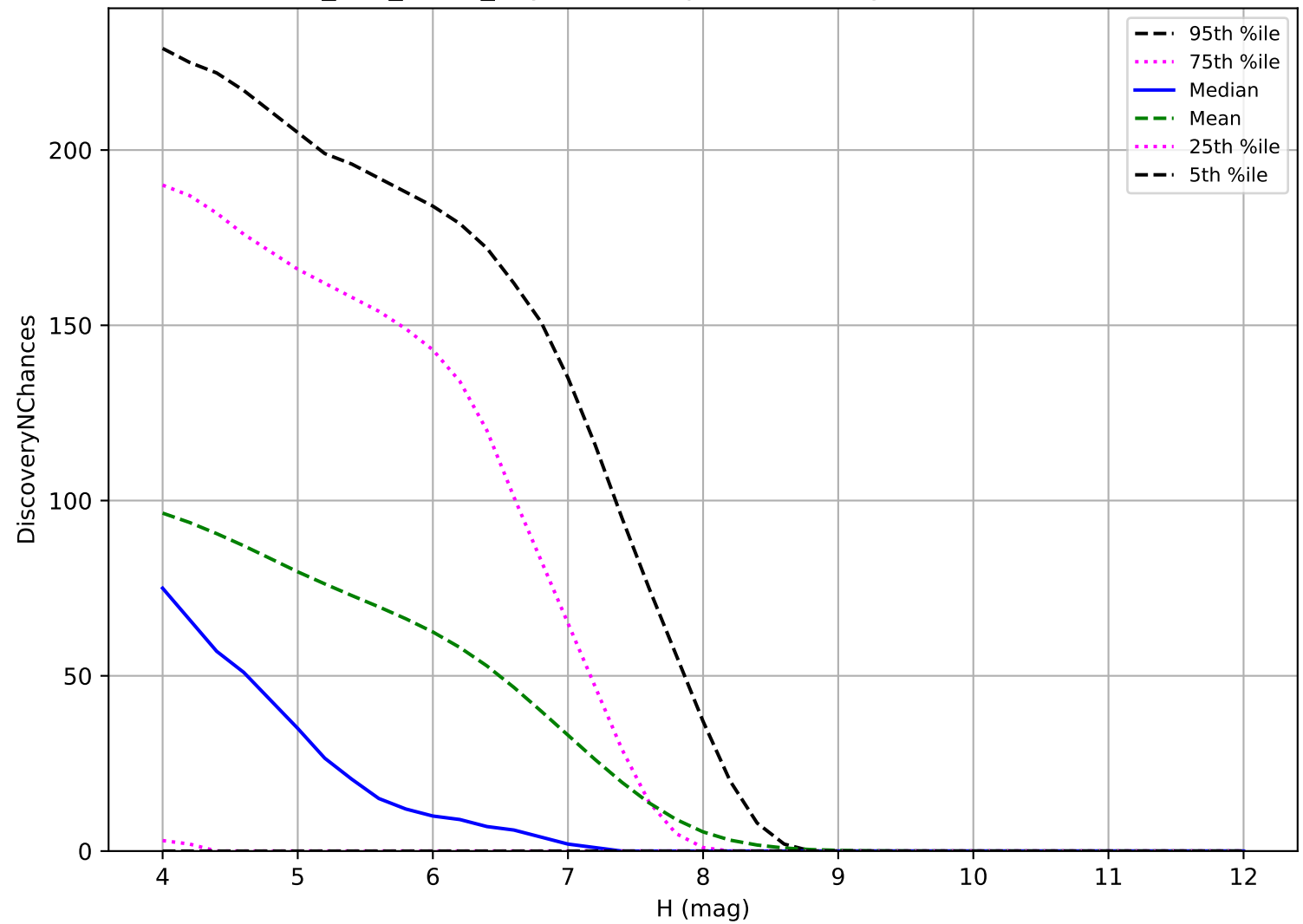
too_100_4v3.4_10yrs: TNO 3 pairs in 15 nights detection loss
