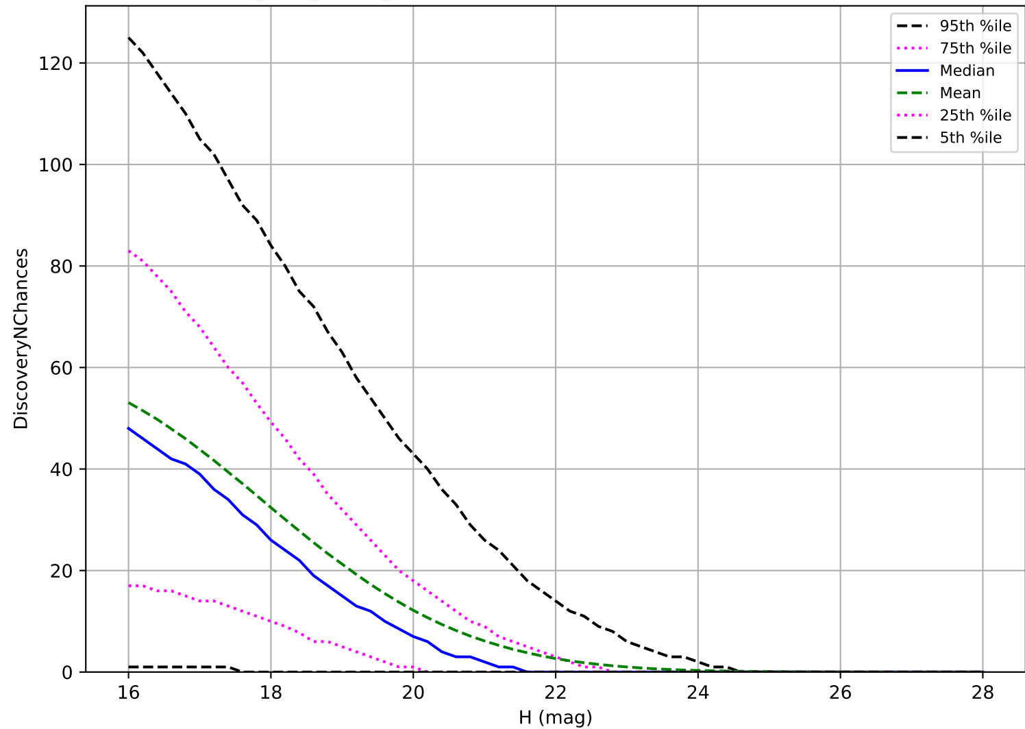
too_100_4v3.4_10yrs: PHA 3 pairs in 15 nights detection loss
