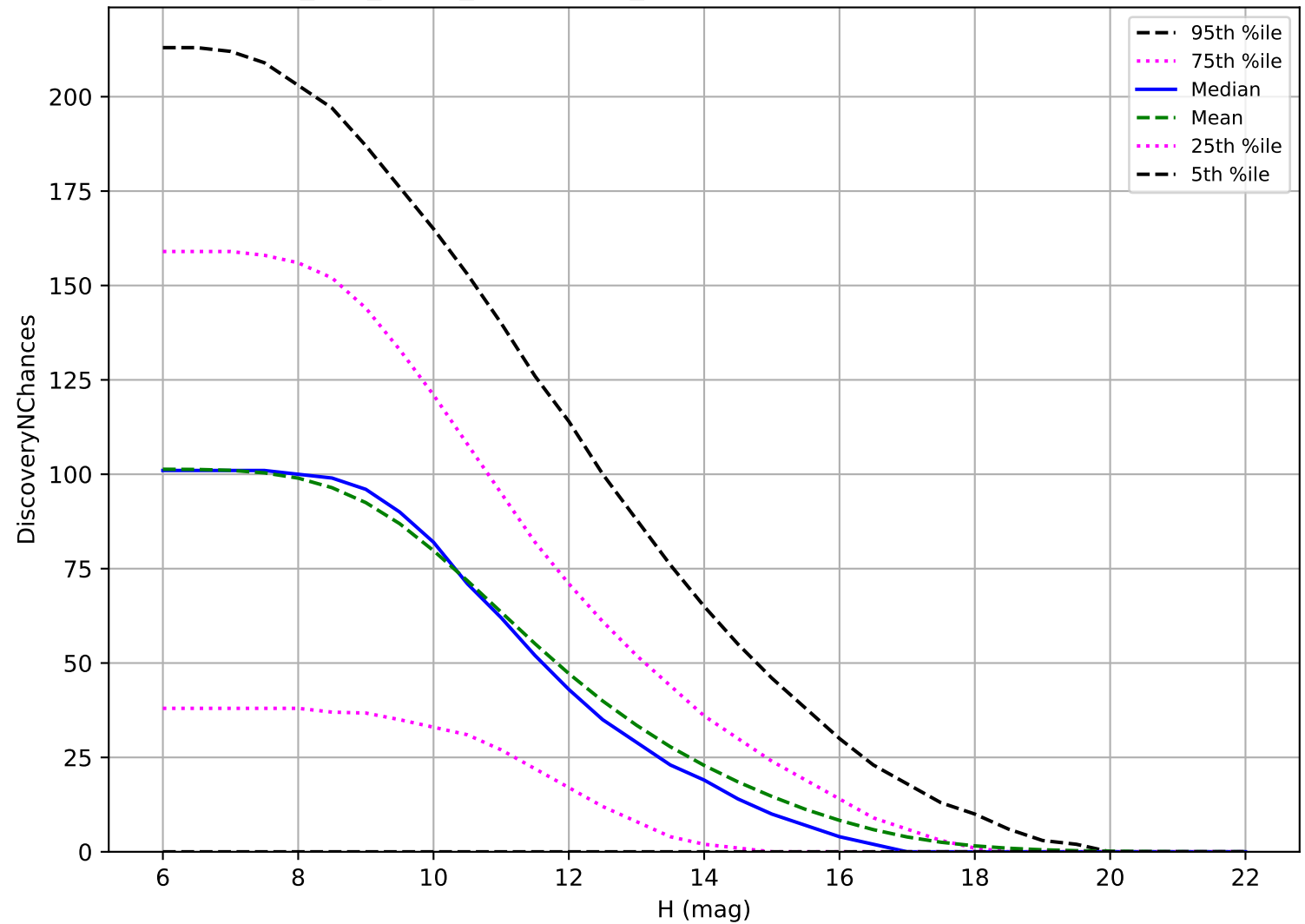
too_100_4v3.4_10yrs: OCC_r5 3 pairs in 15 nights detection loss
