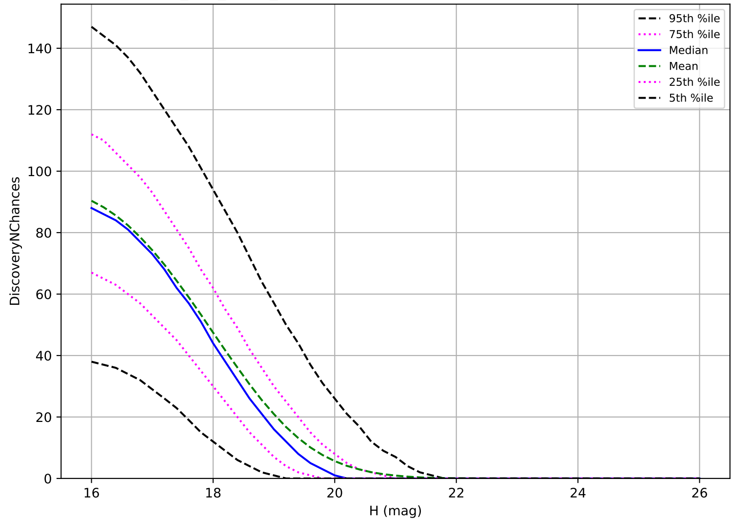
too_100_4v3.4_10yrs: MBA 3 pairs in 15 nights detection loss
