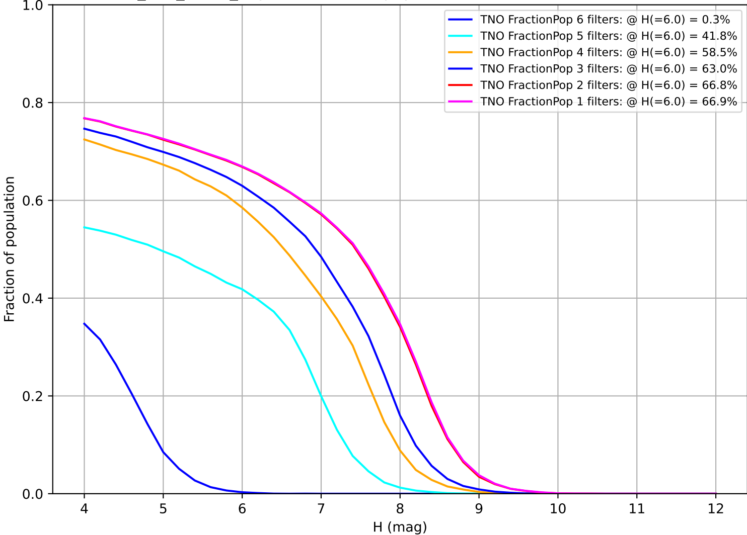
too_100_4v3.4_10yrs: Fraction of population with colors in X filters TNO
