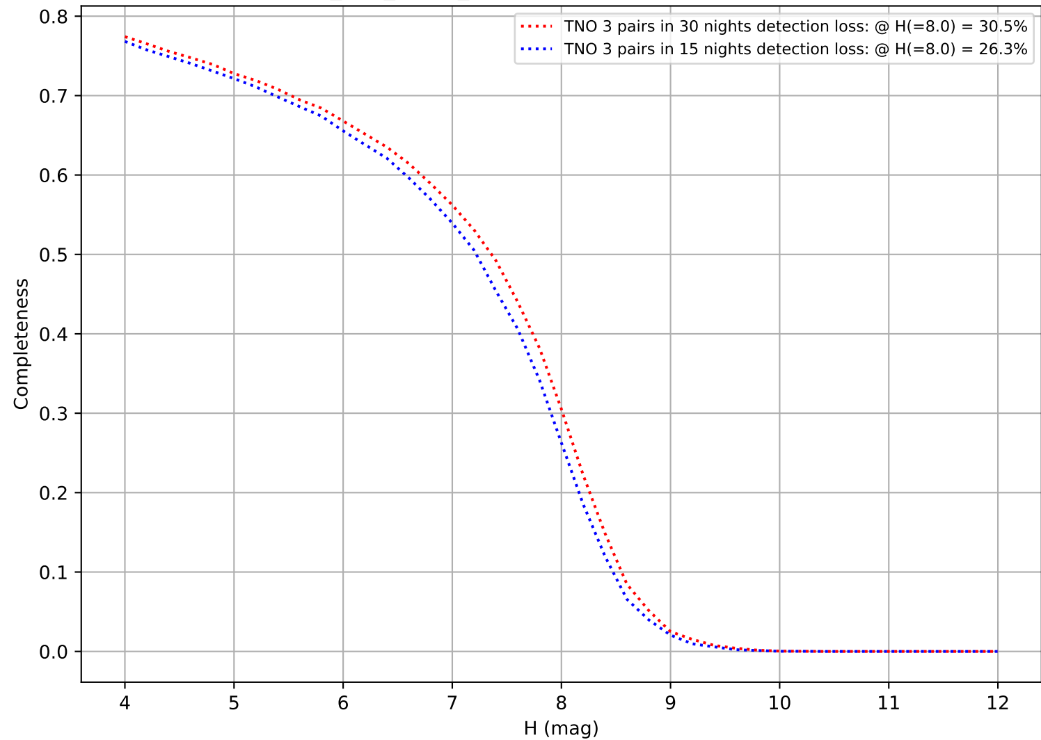
too_100_4v3.4_10yrs: DifferentialCompleteness
