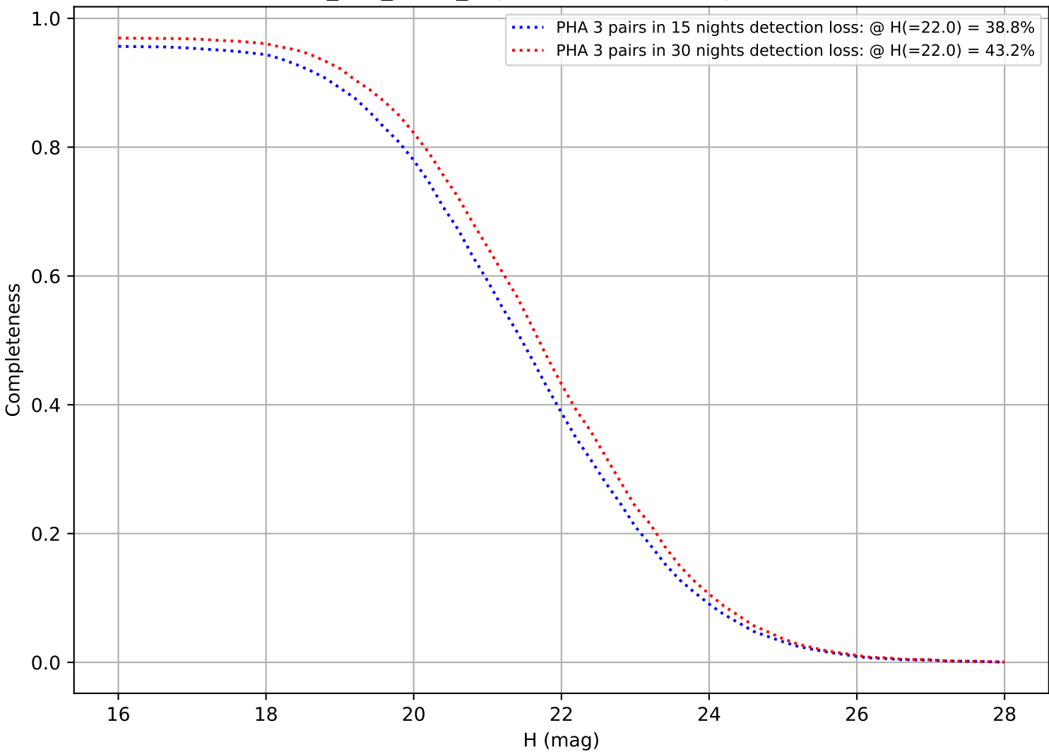
too_100_4v3.4_10yrs: DifferentialCompleteness
