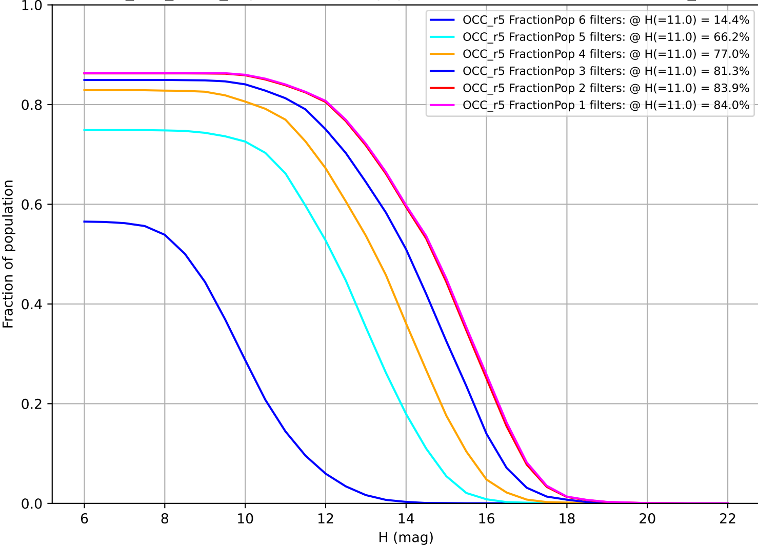
too_100_4v3.4_10yrs: Fraction of population with colors in X filters OCC_r5
