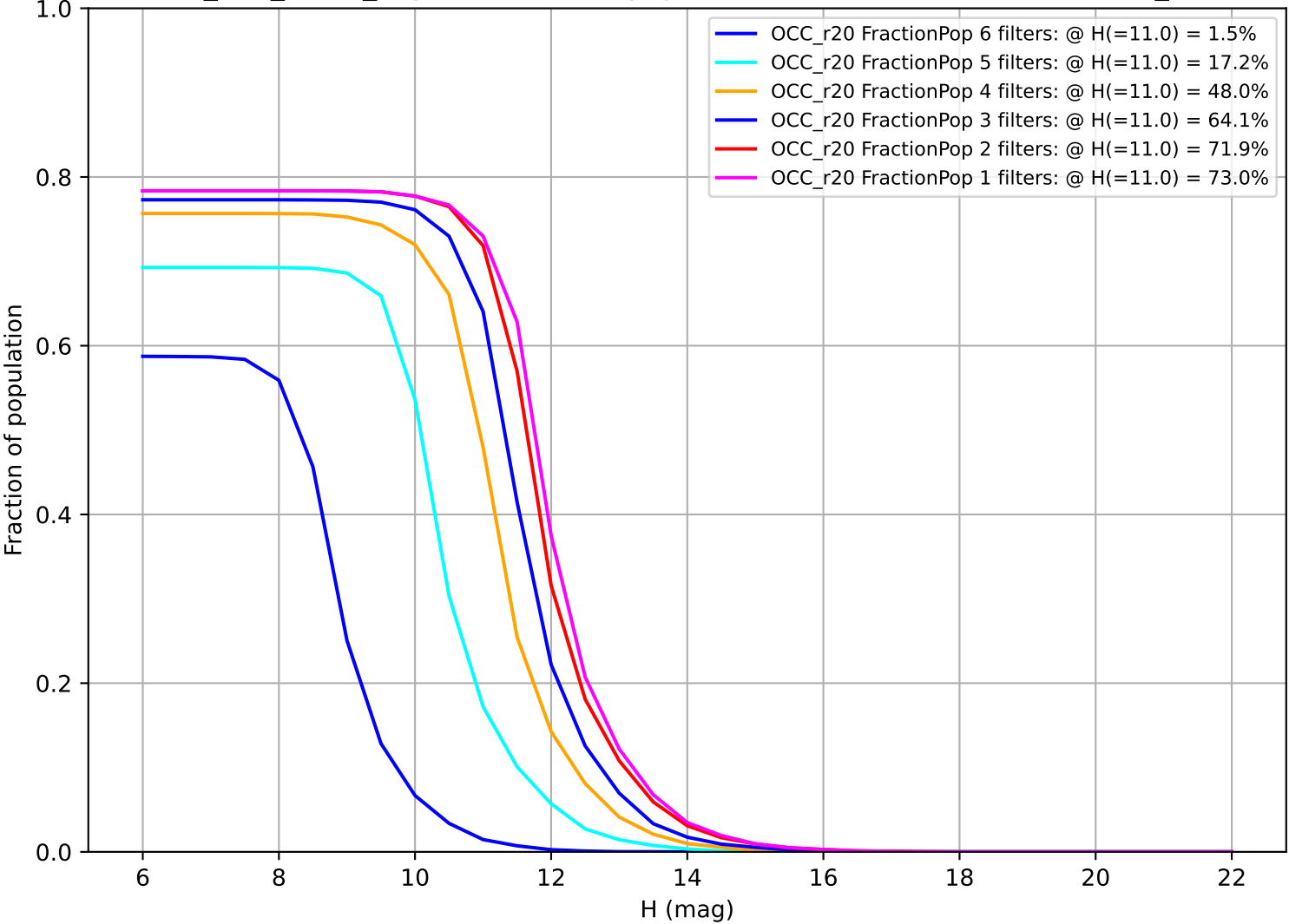
too_100_4v3.4_10yrs: Fraction of population with colors in X filters OCC_r20
